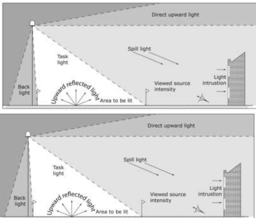
Figure 3.1 Types of obtrusive light
